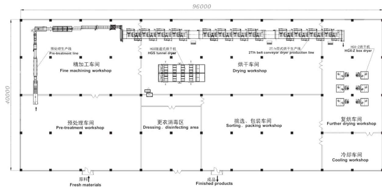
蔬菜烘干车间示意图 Vegetable dehydrated processing workshop diagram
