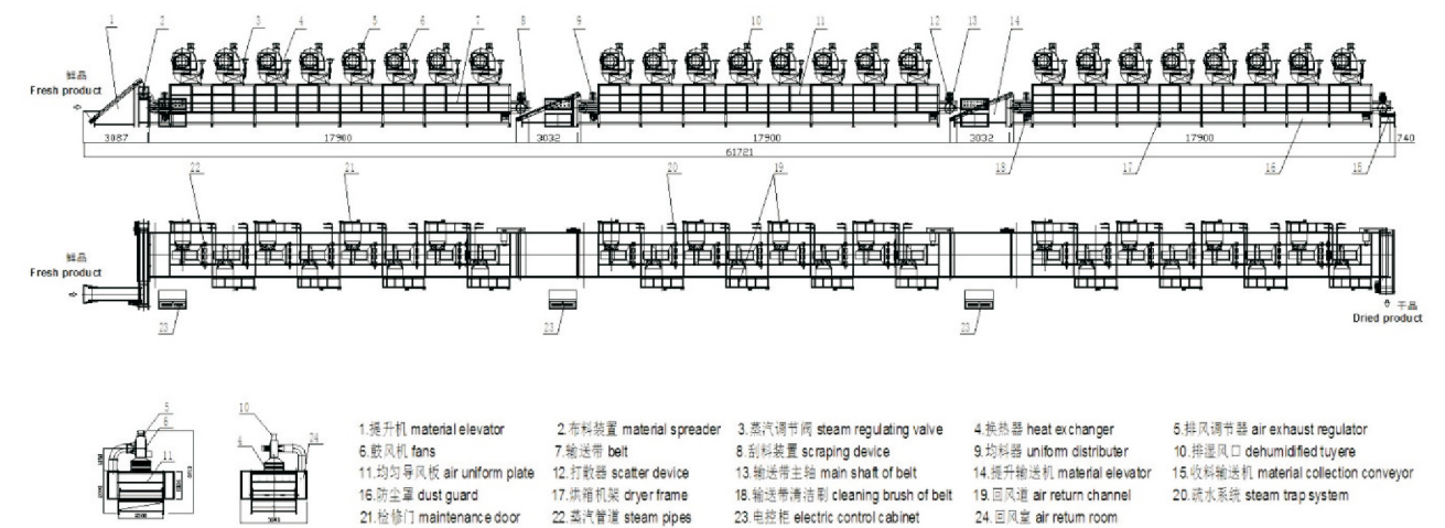
2.5T/h新鲜胡萝卜粒烘干生产线(HGD-2S-32型单层烘干机组合) 2.5T/h fresh carrot granules drying line(HGD-2S-32 single layer drying machines unit)
